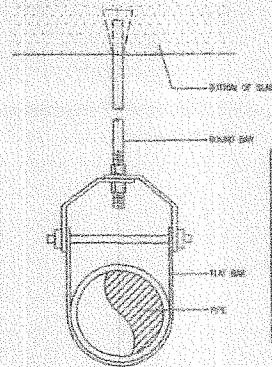
1 ADJUSTABLE CLEVIS PIPE HANGER
