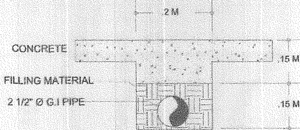
2 DETAIL OF EXCAVATION
